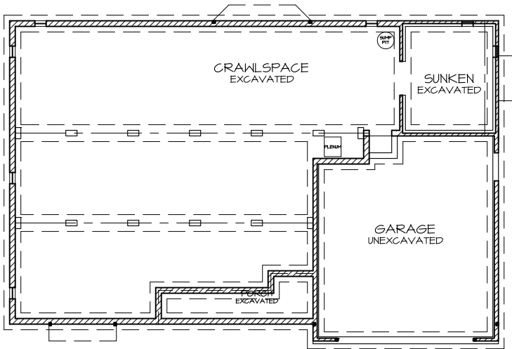
1 FOUNDATION PLAN A-3
